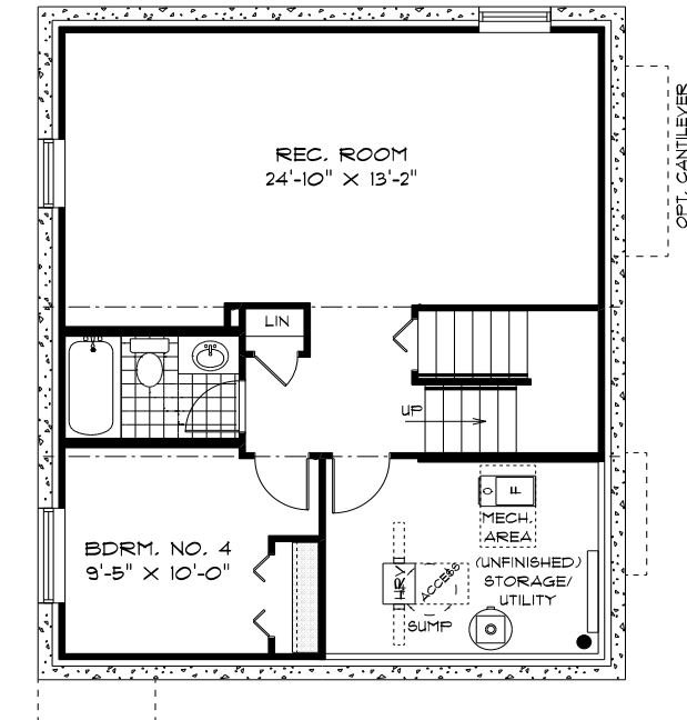
OPTIONAL LOWER LEVEL FLOOR PLAN
